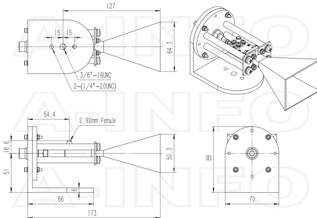
2.92mm Female Output with L Type Mounting Bracket (Option, P/N: LB-42-10-C-MBL)
