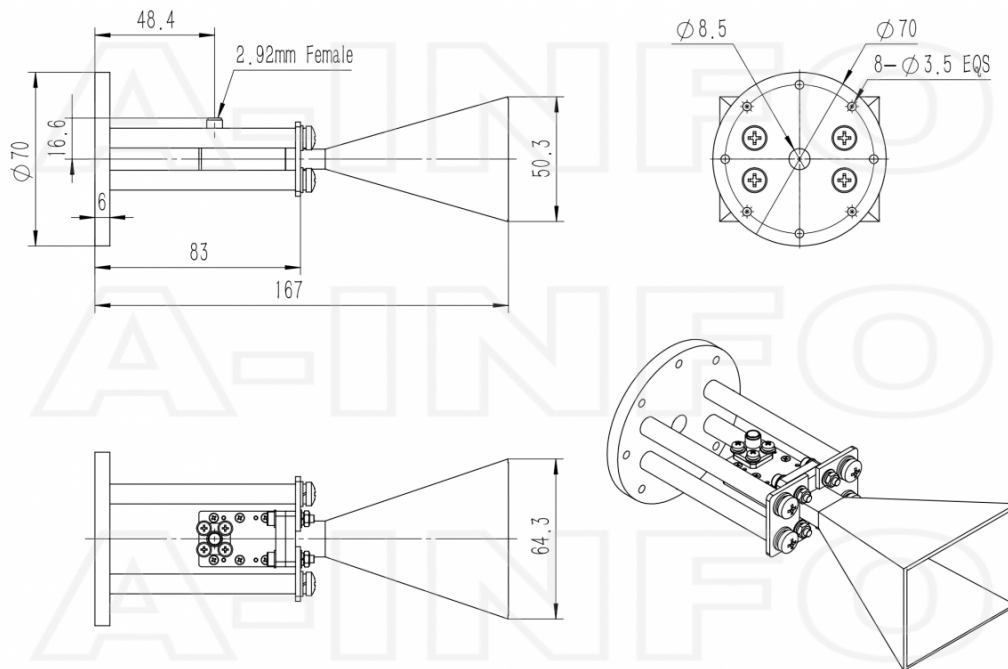
2.92mm Female Output with Round Mounting Bracket (Option, P/N: LB-42-10-C-MB)
